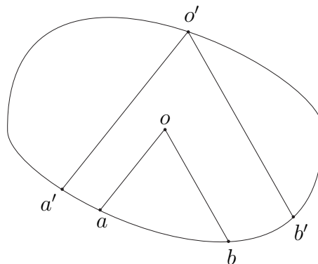
Figure 1. Notation in the proof of Theorem 2
