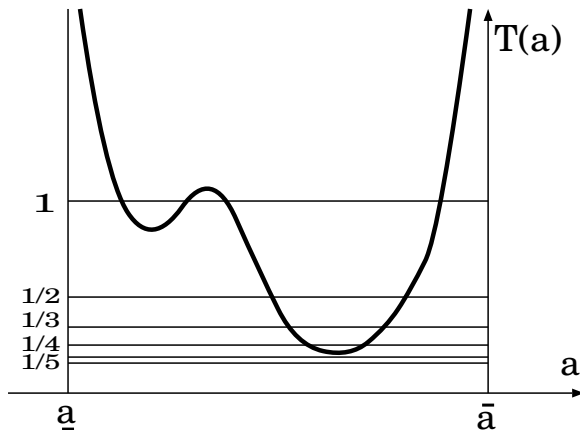
FIGURE 7. The picture shows the graph of T(a) in the case of C_{kl} ( k \neq l ). Each of the intersections of the curve and the lines corresponds to a rotating wave. In this case, the sequence of modified Morse indices is (2, 2, 2, 4, 6, 8, 8, 6, 4, 2) .
