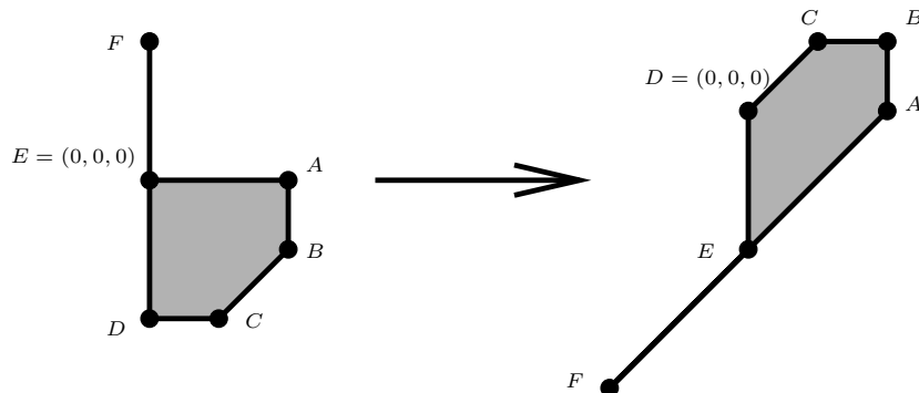
Figure 5: A demonstration of tropical polytope duality.
