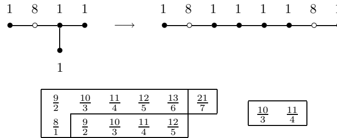
Figure 8: Type D_\ell decomposition, m_{\ell-1} = m_\ell
