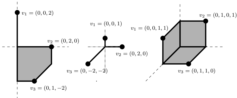
Figure 2: Three tropical polytopes. The first two live in \mathbb{TP}^2 , the last in \mathbb{TP}^3 .
