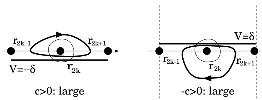
FIGURE 4. The phase planes of (3.2) for two extreme cases. Circles in each picture are the closed orbit corresponding to (a_0, c_0) . If c is large, then the arc corresponding to (a, c) ( a < a_0 ) cannot pass the segment (r_{2k-1}, r_{2k+1}) \times \{-\delta\} and the arrival point is in the inside of the closed orbit (the left picture). If -c is large, then the arc corresponding to (a, c) does not pass the segment (r_{2k}, r_{2k+1}) \times \{0\} (the right picture).
