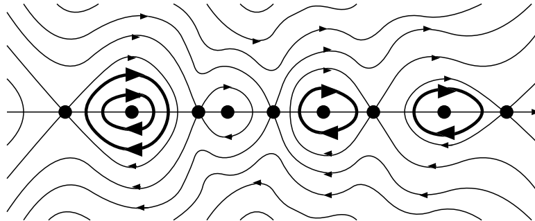
FIGURE 12. The picture indicates the phase portrait when G(p) is as shown in the center of Figure 11. The thick closed curves indicate the closed orbits which correspond to standing waves, and the points indicate equilibrium points which correspond to constant steady states.
