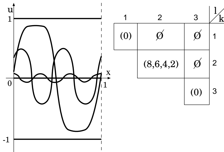
FIGURE 1. Wave profiles (left) and the structure of S (right) for equation (2.4). The three horizontal lines indicate constant steady states.
