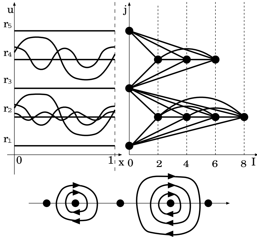
FIGURE 9. In the left figure, the thick curves and the lines indicate the profile of all the waves that move to the right or the left at each constant speed. In the right figure, the horizontal axis indicates the modified Morse index and the vertical axis indicates the suffix of C_{jj} . The points mean elements of S . The thick curves and the lines represent the connecting orbits. The lower figure shows closed orbits and equilibrium points in the uu_x -plane. Note that they do not necessarily correspond to the same value of c .
