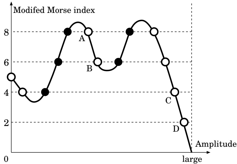
FIGURE 10. Each black point indicates a wave whose Morse index is even (i.e. i(u_j^{kl}) = I(u_j^{kl}) ) and each white point indicates a wave whose Morse index is odd (i.e. i(u_j^{kl}) = I(u_j^{kl}) - 1 ). The point A connects only to B, C, D and two constant steady states.
