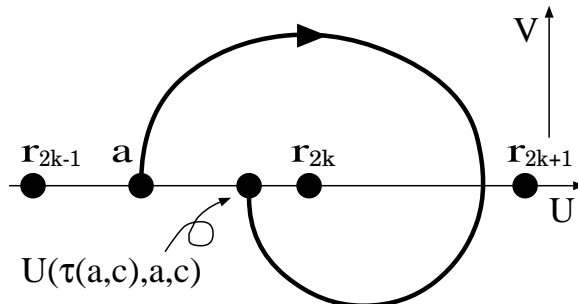
FIGURE 3. The picture denotes the arc that starts from the point (a, 0) at the time 0 and arrives at a point (b, 0) ( r_{2k-1} < b < r_{2k} ) at a certain positive time. The U -coordinate of the arrival point is denoted by U(\tau(a, c), a, c) whose meaning is specified below. The arc deforms with respect to a and c . If we select suitable a and c , then the arrival point coincides with the starting point (i.e. U(\tau(a, c), a, c) = a ), which means the arc is a closed orbit.
