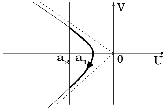
FIGURE 5. This picture indicates the phase plane displayed in the new coordinate. The thick curved arrow (\tilde{U}, \tilde{V}) is the arc that we observe. Two dashed lines are directions of the two eigenvectors of the matrix. The time required for traveling through the thick part of the arc diverges as a_1 \rightarrow 0 .
