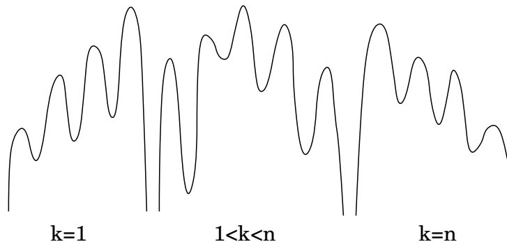
FIGURE 11. The graph of G(r) ; k = 1 (left), 1 < k < n (center) and k = n (right).
