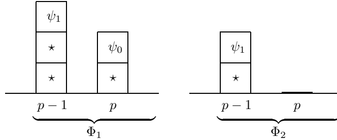
Figure 2: Example of a non-proper asymptotic type
