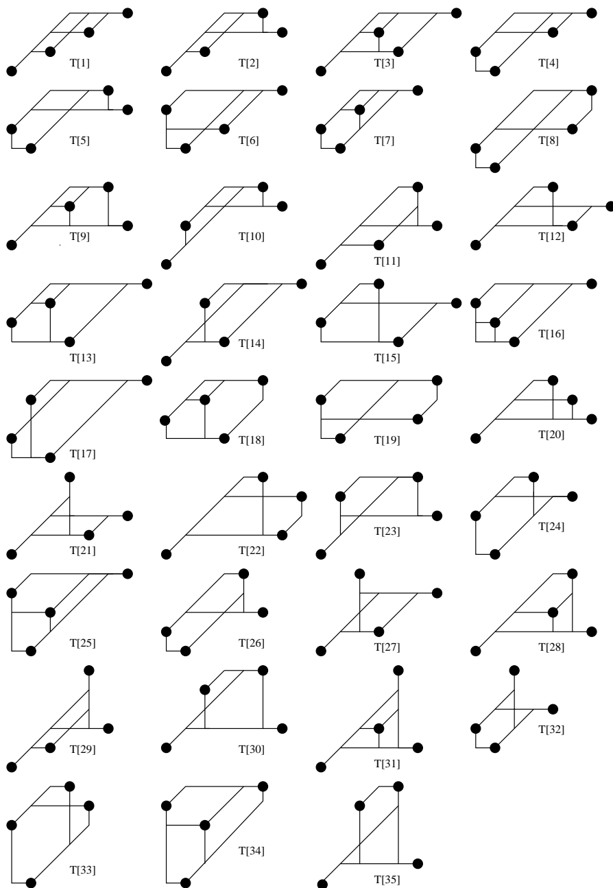
Figure 6: The 35 symmetry classes of tropical complexes generated by four points in \mathbb{TP}^2 .
