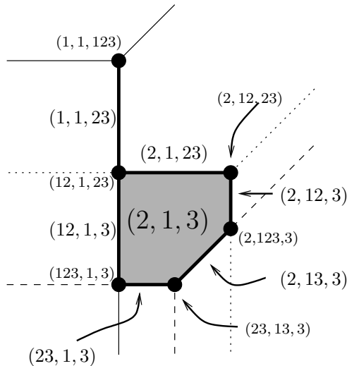
Figure 4: A tropical complex expressed as the bounded cells in the common refinement of the fans v_1 - \mathcal{F} , v_2 - \mathcal{F} and v_3 - \mathcal{F} . Cells are labeled with their types.
