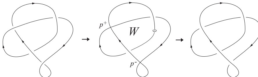
Figure 15: Moving into B^4 from left to right: A trefoil knot in S^3 (left) bounds an immersed disk having a single pair of self-intersections p^\pm admitting a Whitney disk W containing a single order 1 intersection point (center). An unknotted ‘slice’ of the immersed disk is shown on the right. The rest of the immersed disk is described by a null isotopy further into B^4 (not shown) of this unknot.
