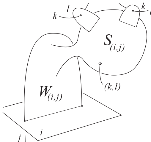
Figure 18: Changing the interior of W_{(i,j)} to W'_{(i,j)} corresponds to tubing W_{(i,j)} into a 2-sphere S_{(i,j)} . Only intersections which contribute to the difference \lambda_2(\mathcal{W}) - \lambda_2(\mathcal{W}') \in \Lambda_2(4) are shown.
