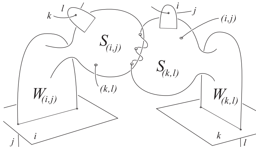
Figure 19: A schematic illustration of how order 0 intersections between S_{(i,j)} and S_{(k,l)} can contribute order 2 indeterminacies. (Only relevant intersections are shown.)
