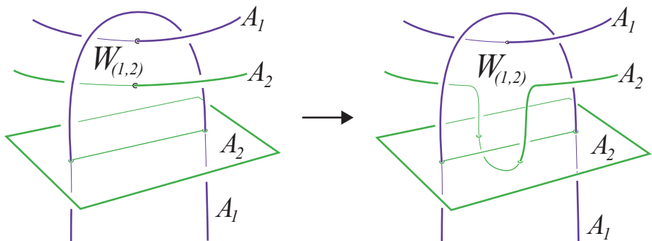
Figure 2: Pushing an intersection between A_2 and the interior of a Whitney disk W_{(1,2)} down into A_2 only creates (two) self-intersections in A_2 .
