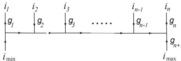
Figure 6: A simple order n tree with minimal- and maximal-labeled vertices connected by a length n+1 geodesic; 1 \leq i_{\min} < i_{\max} \leq m , and i_{\min} < i_k < i_{\max} for 1 \leq k \leq n . Vertex orientations are induced by the planar embedding. By the HOL relations, all but n+1 of the edge decorations can be set to the trivial element in \pi (indicated by the ‘empty-labeled’ edges in the figure).
