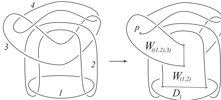
Figure 11: Moving radially into B^4 from left to right, a link L \subset S^3 bounds an order 2 (non-repeating) Whitney tower \mathcal{W} : The order 0 disk D_1 consists of a collar on L_1 together with the indicated embedded disk on the right. The other three order 0 disks in \mathcal{W} consist of collars on the other link components which extend further into B^4 and are capped off by disjointly embedded disks. The order 1 Whitney disk W_{(1,2)} pairs D_1 \cap D_2 , and the order 2 Whitney disk W_{((1,2),3)} pairs W_{(1,2)} \cap D_3 , with p = W_{((1,2),3)} \cap D_4 the only unpaired intersection point in \mathcal{W} . See Figure 12 for the tree-preserving resolution of \mathcal{W} to a grope.
