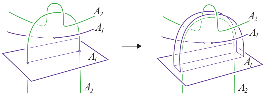
Figure 3: A Whitney move guided by the Whitney disk of Figure 2. The intersection between A_1 and the interior of the Whitney disk becomes a pair of self-intersections of A_1 after the Whitney move.
