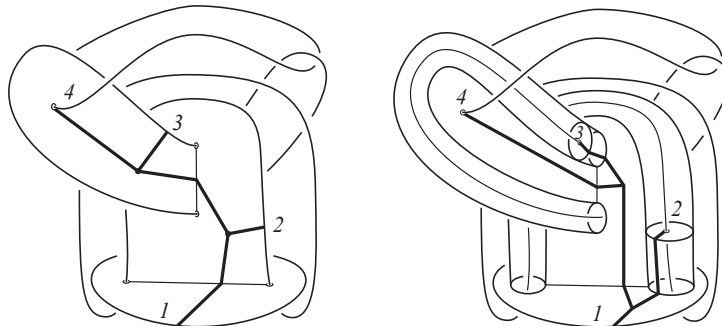
Figure 12: Both sides of this figure correspond to the slice of B^4 shown in the right-hand side of Figure 11. The tree t_p = \langle\langle(1,2),3\rangle,4\rangle \subset \mathcal{W} is shown on the left. Replacing this left-hand side by the right-hand side illustrates the construction of a class 3 (capped) grope G_1^c bounded by L_1 , shown (partly translucent) on the right, gotten by surgering D_1 and W_{(1,2)} . Each of the disks D_2 , D_3 and D_4 has a single intersection with a cap of G_1^c , with G_1 displaying the longitude of L_1 as the triple commutator [x_2, [x_3, x_4]] in \pi_1(B^4 \setminus \mathcal{W}^1) , where \mathcal{W}^1 = D_2 \cup D_3 \cup D_4 . This simple case illustrates the local picture of the general computation of \eta_n^i(\lambda_n(\mathcal{W})) : For a more complicated L = \partial\mathcal{W} this construction would be carried out in a 4–ball neighborhood of each tree containing an i -labeled vertex, and \mathcal{W}^i would consist of other Whitney disks as well as the D_{j \neq i} .
