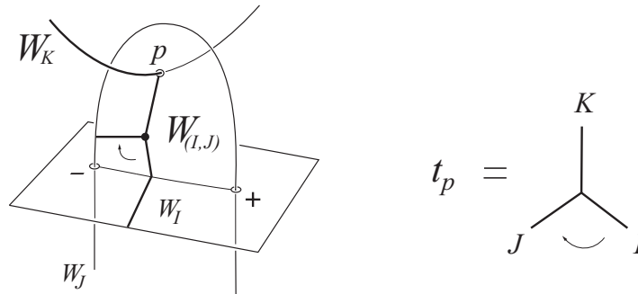
Figure 4: A local picture of the tree t_p = \langle (I, J), K \rangle associated to p \in W_{(I,J)} \cap W_K near a trivalent vertex adjacent to the edge of t_p passing through an unpaired intersection point p in a Whitney tower \mathcal{W} . On the left t_p is pictured as a subset of \mathcal{W} , and on the right as an abstract labeled vertex-oriented tree. In a non-simply connected 4-manifold X the edges of t_p would also be oriented and labeled by elements of \pi_1 X (as in Figure 5 below).
