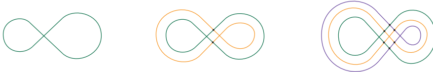
Figure 1: One self-intersection leads to m^2 - m intersections among m copies.
