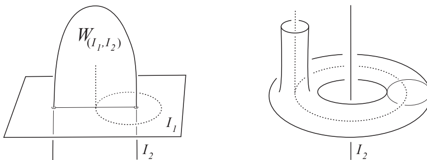
Figure 9: The normal circle bundle T_I to W_{I_1} and W_{(I_1, I_2)} over the dotted circle and arc on the left is shown on the right.
