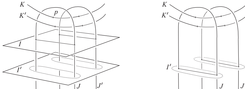
Figure 7: Extending a Whitney tower using parallel Whitney disks: An unpaired intersection point p \in W_{(I,J)} \cap W_K in a Whitney tower on A , where each of I , J and K contain exactly one occurrence of the index m , gives rise to eight unpaired intersections in four Whitney disks in the new Whitney tower on A' , formed from A by including a parallel copy of A_m . The dotted oval loops (left) bound neighborhoods of the Whitney arcs in the opaque I' sheet which have been perturbed into a nearby time coordinate along with the two corresponding translucent Whitney disks (right).
