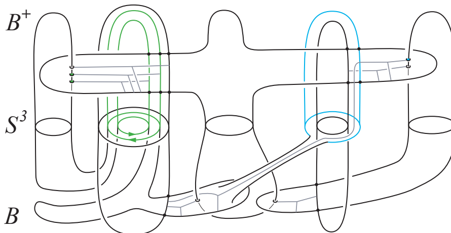
Figure 14: The non-repeating Whitney tower \mathcal{V} = \mathcal{W}^+ \cup \mathring{\mathcal{W}}' \subset S^4 = B \cup_{S^3} B^+ : The links L \subset L' \subset S^3 are shown in the horizontal middle part of the figure. The components of L are black; the component of L^1 \subset L' is blue, and an oppositely oriented pair of components in L^0 \subset L' are shown in green. The lower part of the figure shows \mathring{\mathcal{W}}' \subset B , and the upper part shows \mathcal{W}^+ \subset B^+ . The tree shown involving the blue L^1 -component passes down through L^1 into a Whitney disk of \mathring{\mathcal{W}}' and then down into a pair of order 0 disks in \mathring{\mathcal{W}}' , so the tree is of order greater than n . The pair of trees each having a univalent vertex on a green order 0 disk in \mathcal{W}^+ have opposite signs due to the opposite orientations on the green disks.
