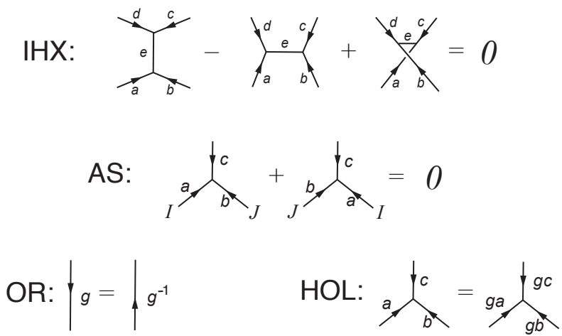
Figure 5: The relations in \mathcal{T}_n(\pi, m) : IHX (Jacobi), AS (antisymmetry), OR (orientation), HOL (holonomy). These are ‘local’ pictures, meaning that the unlabeled univalent vertices extend to fixed decorated subtrees in each equation. For instance, in the right-hand term of the HOL relation only the three visible edge decorations are multiplied by the element g , corresponding to a change of whisker on a Whitney disk at the indicated trivalent vertex. All vertex-orientations are induced from a fixed orientation of the plane; in particular, the two terms in the AS relation only differ by the orientation at the indicated trivalent vertex, where the two edges extending to the subtrees I and J have been interchanged.
