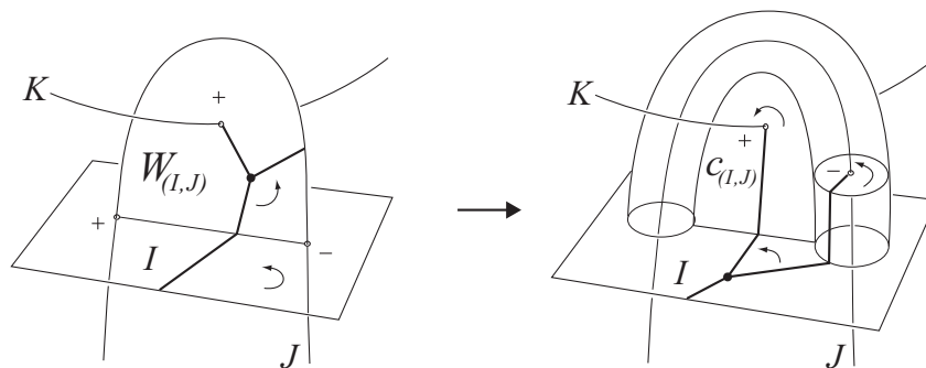
Figure 13: Resolving a Whitney tower to a capped grope preserves the associated oriented trees. The boundary of the I -labeled sheet represents the commutator [x_J, x_K] , up to conjugation, of the meridians x_J and x_K to the J - and K -labeled sheets.
