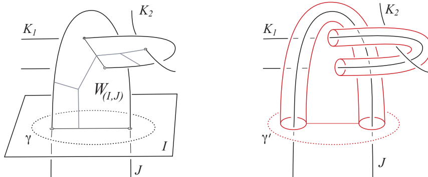
Figure 10: Left: A (dotted) oval \gamma \subset W_I . Right: A (dotted) parallel \gamma' to the oval bounds a grope in a nearby ‘time’ coordinate. Not shown is the dual branch of the grope attached to the meridian of W_J (as per Lemma 26).
