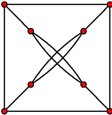
Figure 12: Base graph for girth 17
