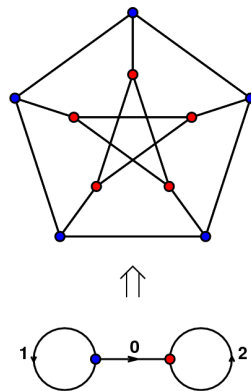
Figure A1: The Petersen graph as a lift
