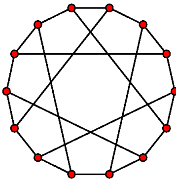
Figure 2: The Heawood graph
