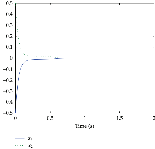
Figure 1: The state x_1 and x_2 of the closed-loop system in Example 4.3.
