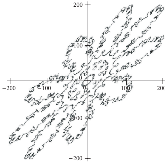
Figure 4.4. a = 2 \cos(2\pi/9) , \theta = 2\pi/9 .
