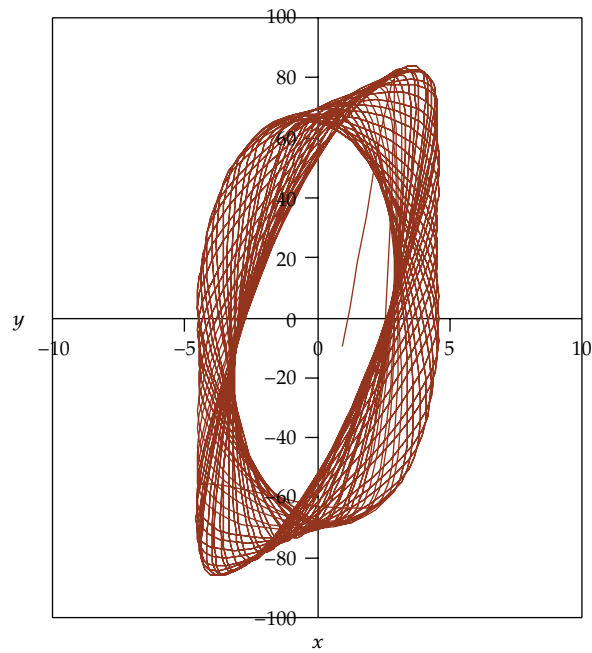
Figure 4: Stable limit cycle of system (3.5) for \alpha = 0.95 , a_1 = 1 , a_3 = -10 , and \varepsilon = 0.001 with starting point (1, 1) .
