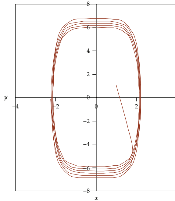
Figure 1: Stable limit cycle of system (3.5) for \alpha = 1 , a_1 = 1 , a_3 = -10 , and \varepsilon = 0.01 with starting point (1, 1) .
