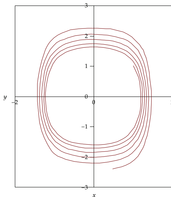
Figure 2: Unstable limit cycle of system (3.5) for a_1 = 1, a_3 = 2, and \varepsilon = 0.01 with starting point (1, 1).
