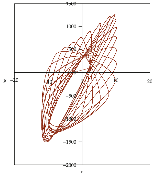
Figure 5: Stable but sensitive limit cycle of system (3.5) for \alpha = 0.945 , a_1 = 1 , a_3 = -10 , and \varepsilon = 0.001 with starting point (1, 1) .
