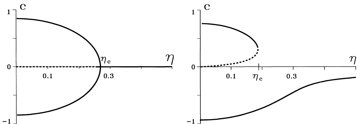
FIGURE 5 Pitchfork front bifurcations showing front solutions of Eq. (5) that propagate at constant velocities, c , as functions of the control parameter \eta = (\epsilon\delta)^{1/2} . The symmetric bifurcation for a_0 = 0 on the left, and the imperfect bifurcation for a_0 = -0.1 on the right.
