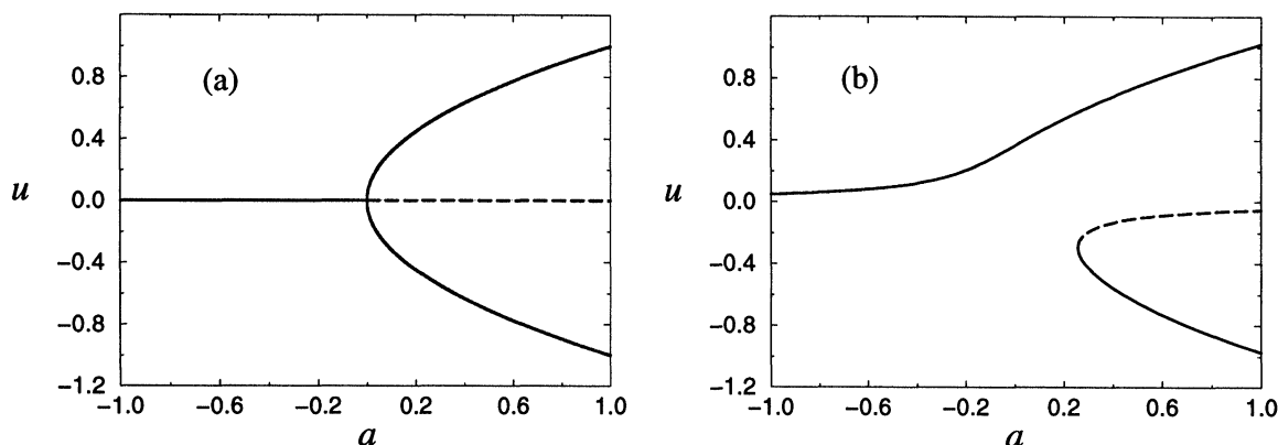
FIGURE 2 A pitchfork bifurcation diagram showing stationary solutions of Eq. (1) as functions of the control parameter a . (a) The symmetric case, b=0 . (b) The asymmetric or imperfect case, b=0.05 .
