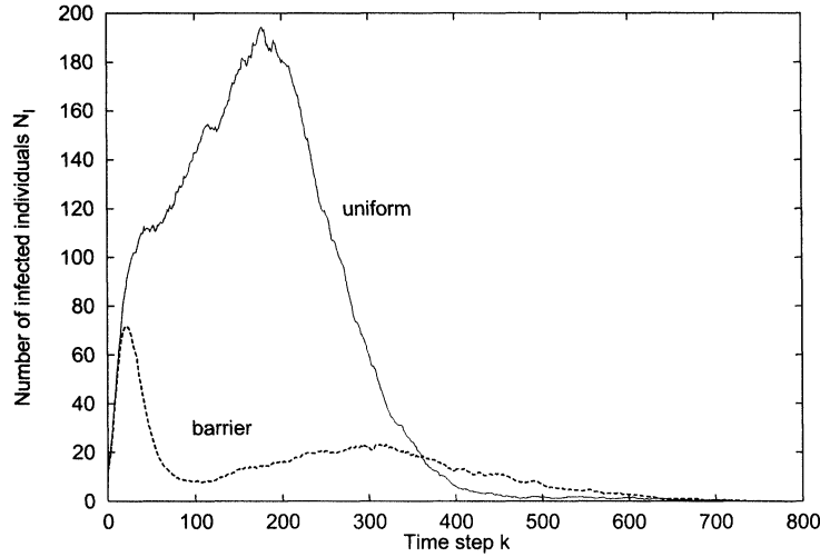
FIGURE 4 Number of infected individuals as a function of time, under “uniform” and “barrier” vaccination strategies. Each simulation curve represents average of 100 LGCA experiments. For each type of vaccination strategy each simulation has been performed on a hexagonal lattice with 10^4 nodes with r=0.3 , a=0.2 , and with 16000 susceptibles uniformly and randomly distributed on the lattice at k=0 , and 10 infectives uniformly and randomly distributed in the circle of radius 20 on the lattice at k=0 .
