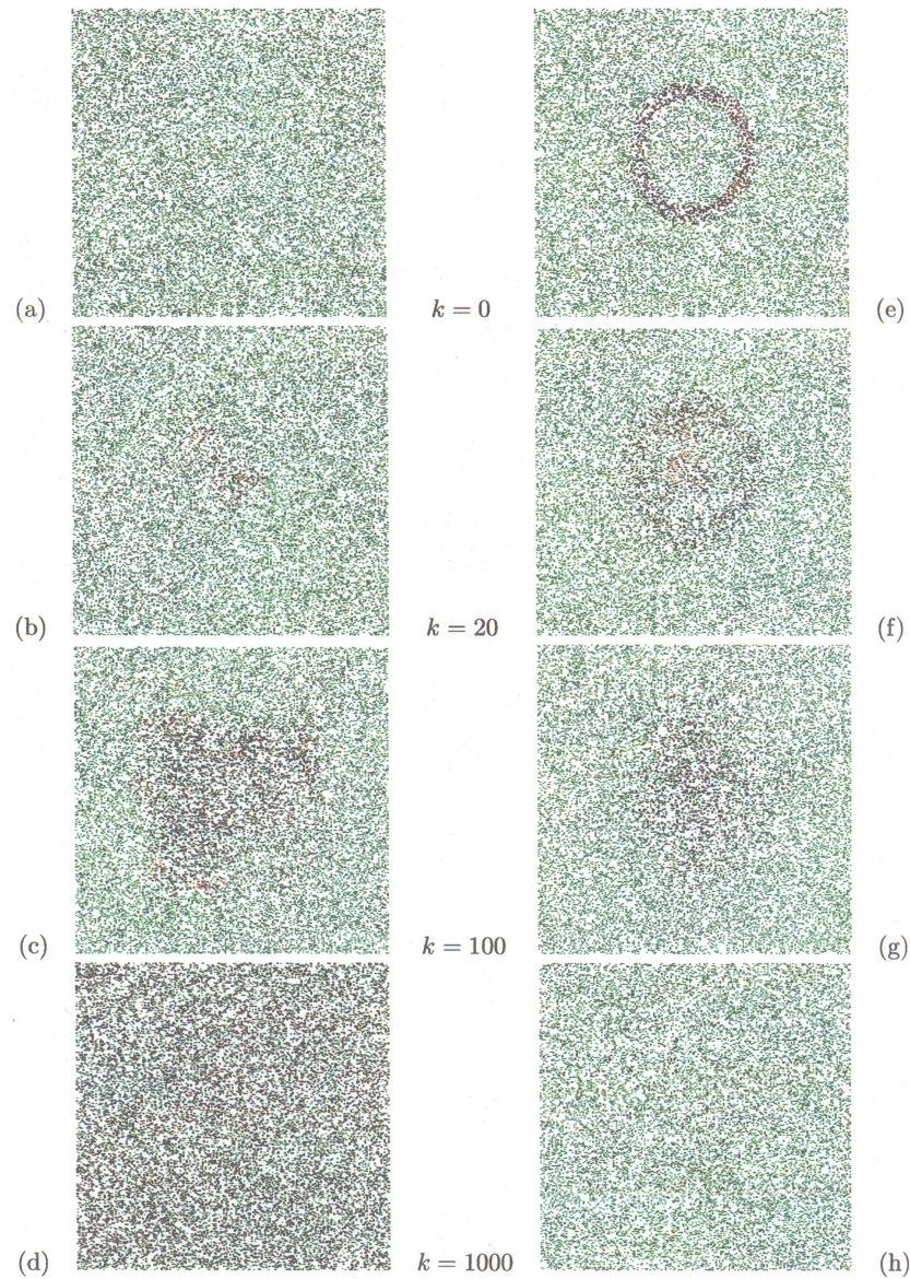
FIGURE 3 Snapshots of LGCA dynamics evolution under “uniform” (left) and “barrier” (right) vaccination strategies. (See Color Plate I.)
