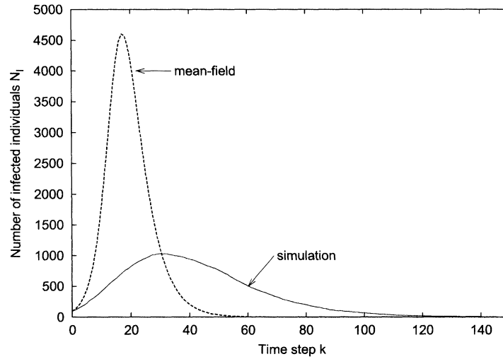
FIGURE 2 Number of infected individuals as a function of time, comparison of LGCA simulation results with the mean-field approximation. The simulation curve represents average of 50 LGCA experiments. Each LGCA simulation has been performed on a hexagonal lattice with 10^4 nodes with r=0.3 , a=0.2 , and with 16000 susceptibles and 100 infected individuals uniformly and randomly distributed on the lattice at k=0 .
