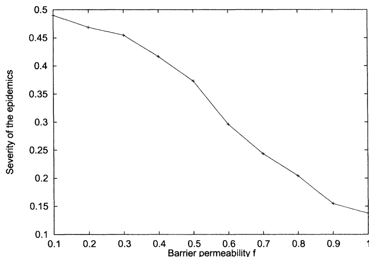
FIGURE 5 Average severity of epidemics of an infectious disease \langle N_R(\infty) - N_R(0) / N_{\text{tot}} \rangle , calculated as average over severities of outbreaks of epidemics of the disease, as a function of barrier permeability f . For each f the average \langle \cdot \rangle has been taken over 100 LGCA simulations of outbreaks of epidemics, each starting with identical initial configuration, and r=0.3 and a=0.2 .
