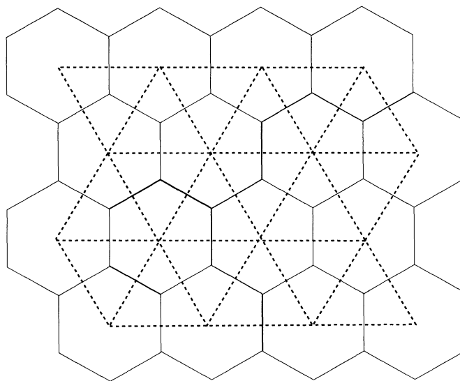
FIGURE 1 The array of hexagonal cells with a dashed lattice superimposed on it. The lattice depicts the channels through which the individuals are transported from cell to cell. The figure is reproduced from Voroney and Lawniczak (2000).
