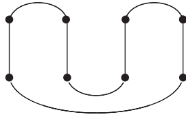
Figure 3: Concatenation {}_aT_b .
