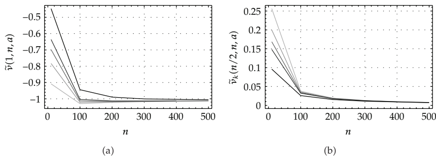
Figure 3: Dependence of \tilde{v}(1, n, a) and \partial\tilde{v}(k, n, a)/\partial k|_{k=n/2} on n for a = 10, 20, 30, 40, 100 . Plots are shown in gray-level intensity, from lower to higher, according to the value of a .
