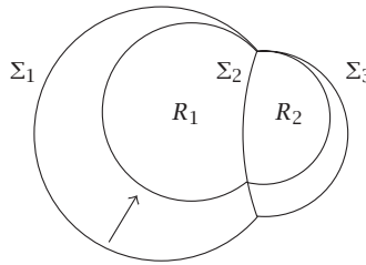
FIGURE 2.2. Increasing the curvature of \Sigma_1 while keeping the curvature of \Sigma_2 fixed increases the curvature of \Sigma_3 . The volumes of R_1 and R_2 both decrease.
