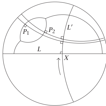
FIGURE 7.6. Generating curve for a possible nonstandard minimizer, and a set of points p_i from which orthogonal lines intersect the same geodesic orthogonal to the axis of revolution orthogonally.
