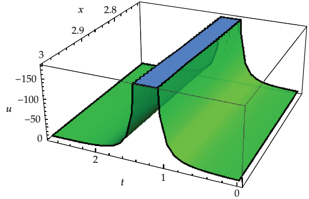
FIGURE 1: Evolution of travelling wave solution (14) with parameters y = 0, \rho = 0.42 .
