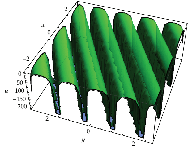
FIGURE 2: Evolution of travelling wave solution (17) with parameters t = 0 , \omega = 0.1 , \rho = -1.53 .
