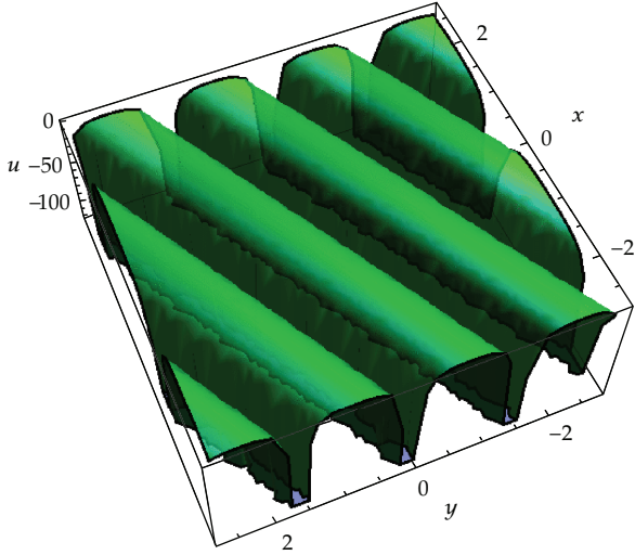
FIGURE 3: Evolution of travelling wave solution (19) with parameters t = 0, \omega = 0.2, \rho = -1.12 .
