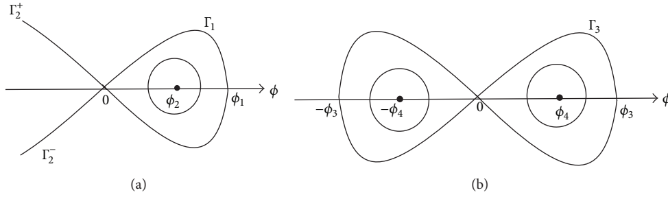
FIGURE 2: The phase portraits of Sy. (16). (a) For p < q , p - q is odd and c > 0 . (b) For p < q , p - q is even and c > 0 .
