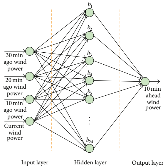
FIGURE 2: The architecture of the proposed RBF neural network based wind power forecasting method.
