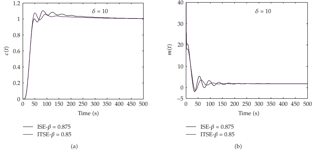
Figure 20: Step responses of the closed-loop system and the controller output for the ISE and the ITSE indices, with a \text{PID}^\beta controller, \delta = 10 and x = 3.0 m.
