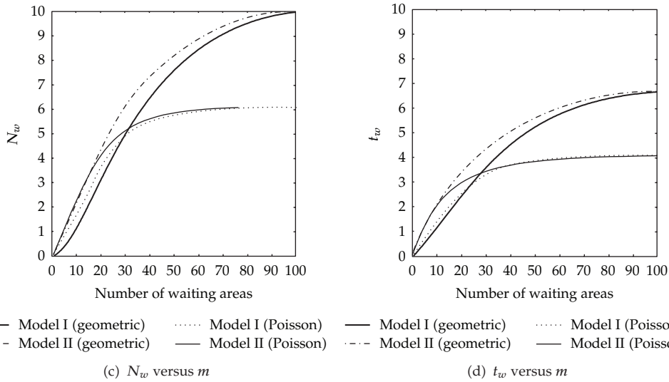
Figure 8: Impact of waiting area size on operating parameters' changes for M^X/M/3/36 queue with different distribution of batch size.
