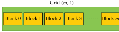
Figure 5: Schematic diagram of Grid ( m, 1 ).
