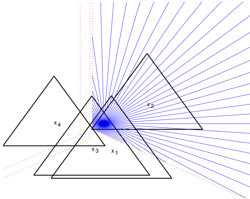
Figure 4: Illustration of the star-shaped property in Lemma 2.9. There are 4 triangles with centers labeled x_1, \dots, x_4 . The triangles centered at x_1, x_2 and x_3 intersect to form another triangle T , and the set \bigcap_{i=1,2,3} S(i|4) , is star-shaped with respect to the barycenter of T . The boundaries of the regions S(i|4) , i = 1, 2, 3 are drawn using dotted lines.
