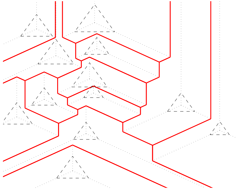
Figure 3: The Voronoi diagram associated with the simplex arrangement in Figure 2. Observe that the boundaries of the Voronoi sets correspond to the dashed line segments in Figure 2 and the solid lines in Figure 2.
