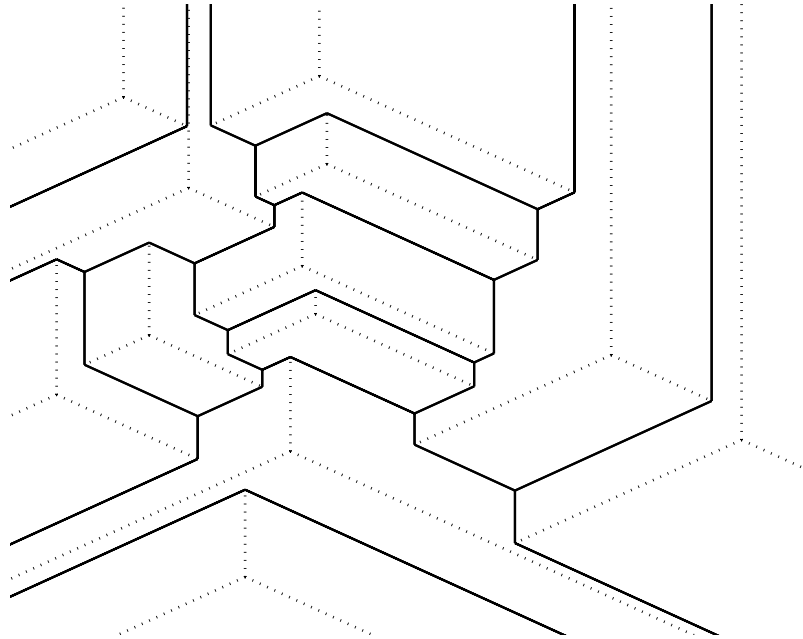
Figure 1: An orthant arrangement. The vertices of the orthants are the points where dotted line segments meet, and the solid line segments show where the orthants share common boundaries.
