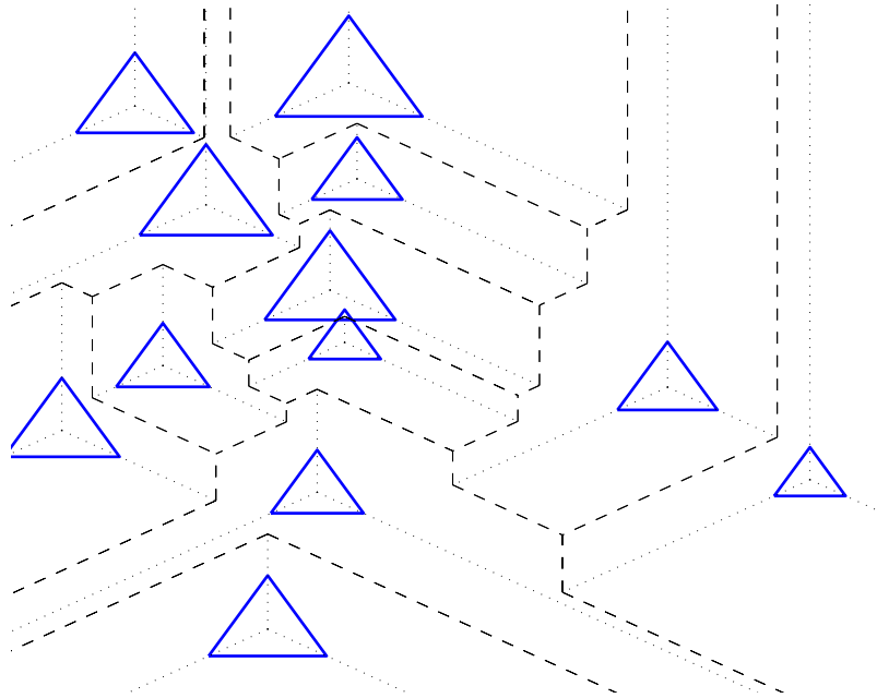
Figure 2: Simplex arrangement obtained by slicing the orthant arrangement in Figure 2 with the hyperplane H .
