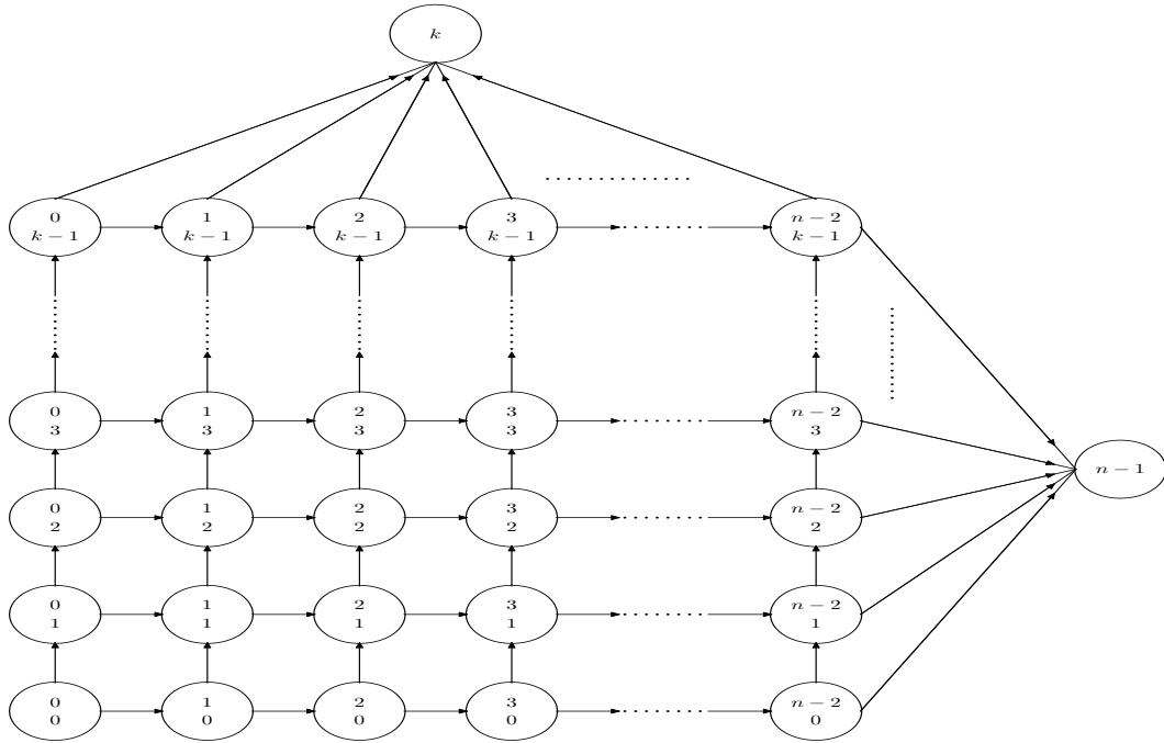
Figure 1: The Markov Process with absorbing states.
