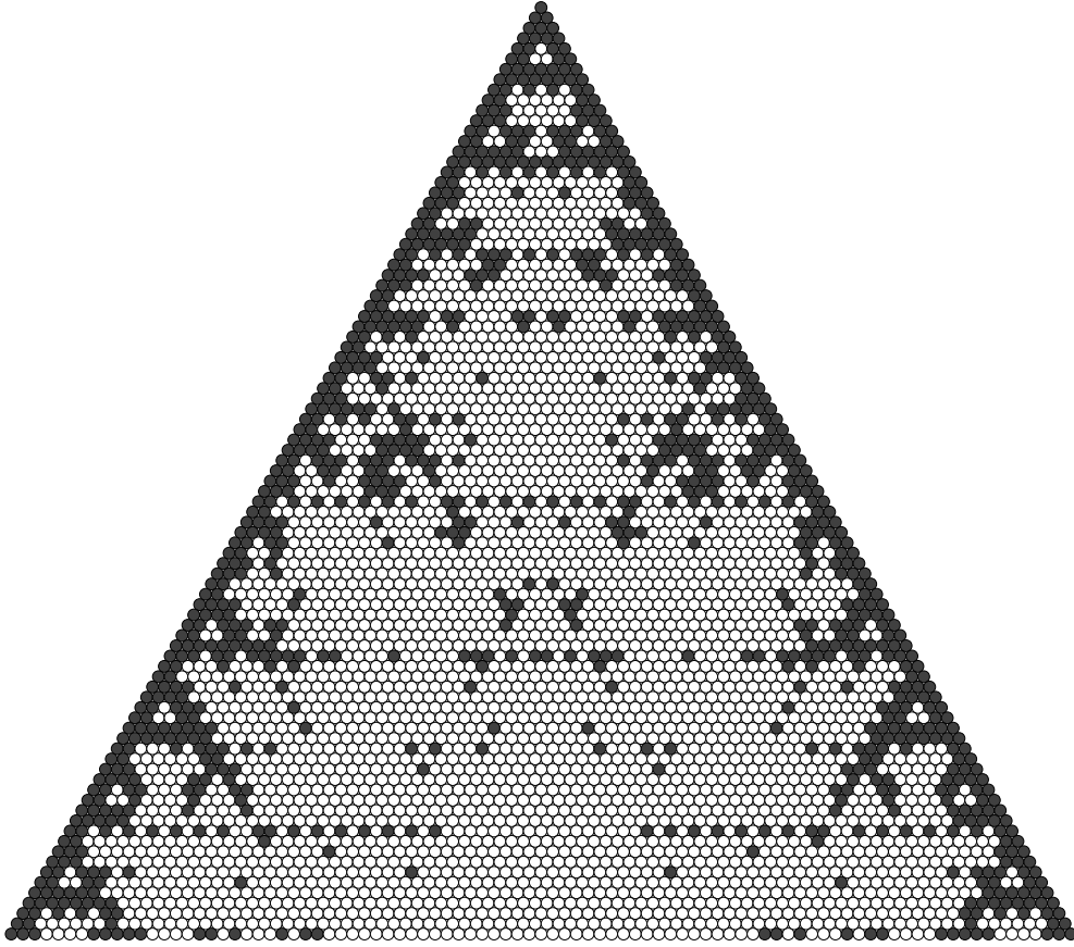
Figure 1: Triangle of values of n and m such that \binom{n+m}{n}_f is always an integer when f is multiplicative.
