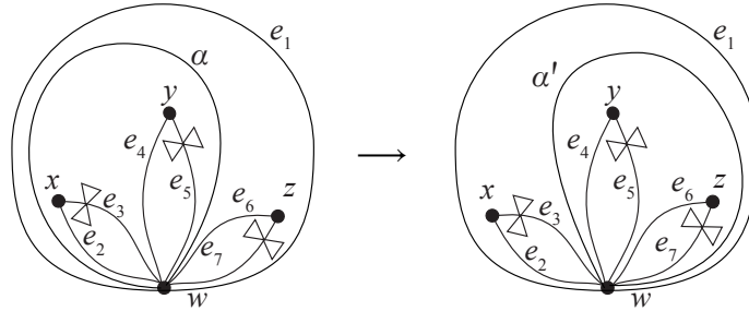
FIGURE 13. In Case 9, two puzzle pieces of type B and C are glued along only one edge \alpha . The exchange relation is \alpha\alpha' = e_1e_4e_5 + e_2e_3e_6e_7 .
