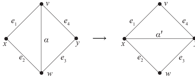
FIGURE 5. In Case 1, two type A puzzle pieces are glued along exactly one edge \alpha . The induced exchange relation from flipping \alpha is \alpha\alpha' = e_1e_3 + e_2e_4
