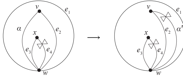
FIGURE 8. In Case 5, a type A puzzle is glued to a type B puzzle along two edges, and we flip the one labeled \alpha . The exchange relation is \alpha\alpha' = e_1 + e_3e_4 .
