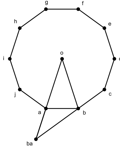
FIGURE 4. Regular decagon (a, b, c, d, e, f, g, h, i, j) with the centre o
