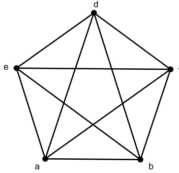
FIGURE 2. Regular pentagon (a, b, c, d, e)
