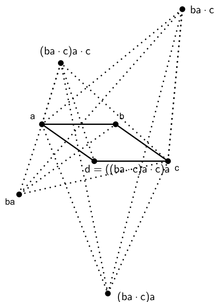
FIGURE 1. Definition of parallelogram
