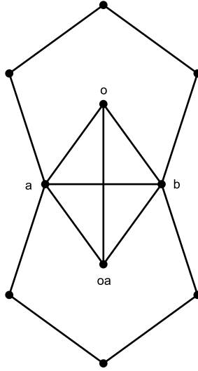
FIGURE 3. Centre of regular pentagon
