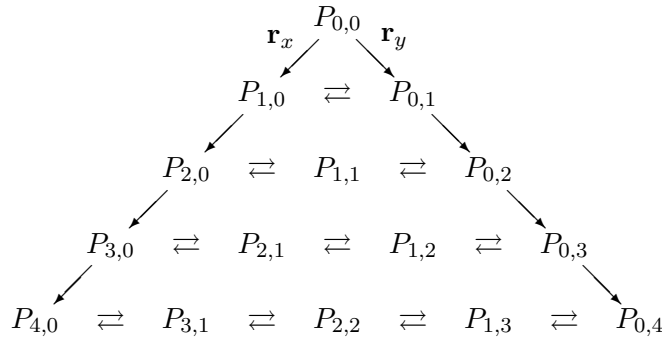
Figure 1. The triangular lattice of polynomials P_{n-k,k} , k = 0, \dots, n with P_{0,0} = 1 , for system (9). Horizontal arrows denote the action of I_1 (left) and I_2 (right).
