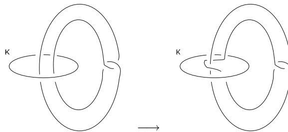
Figure 1: Inequivalent links formed by twisting along unknotted K
