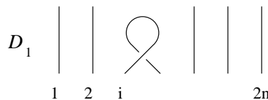
Figure 27: Right-twisted curl in the standard position
