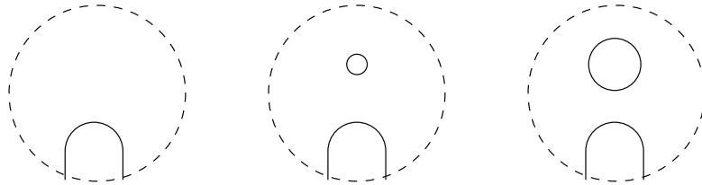
Figure 26: \iota_0 cobordism
