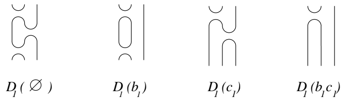
Figure 34: Resolutions of 0-resolution of a_1
