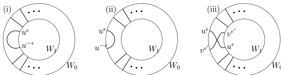
Figure 4: Extending the dissection of D' across the annulus A to a dissection of D = D' \cup A .
