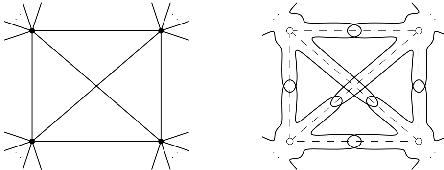
Figure 10: How to modify the construction of the circle diagram for the surface S at each of the self-intersection points in the planar projection of the graph \Delta^{\text{op}} .
