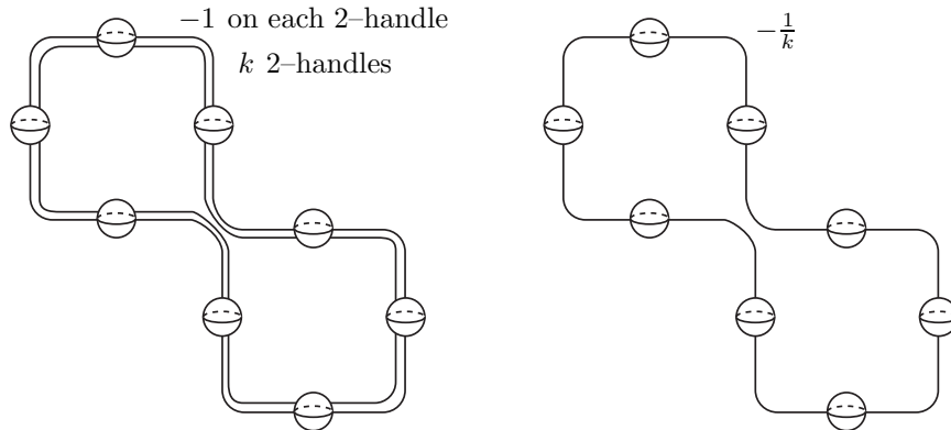
Figure 1: On the left hand side we show an open book with k right handed Dehn twists parallel to the boundary. The right hand side is homeomorphic to the left hand side.
