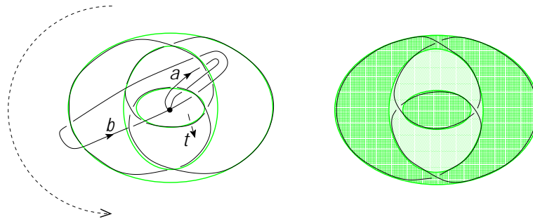
Figure 2: Mutation along the Seifert surface
