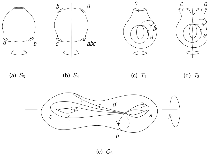
Figure 1: Ruberman's symmetric surfaces: a thrice-punctured sphere S_3 , a four-punctured sphere S_4 , a once-punctured torus T_1 , a twice-punctured torus T_2 and a genus-two surface G_2 along with the shown involutions.
