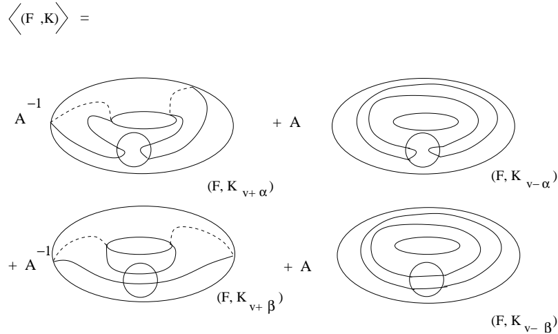
Figure 7: Surface-State Equation
