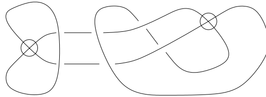
Figure 18: Modified Kishino's Knot
