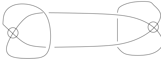
Figure 12: Kishino's Knot
