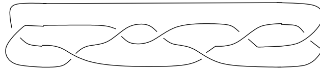
Figure 27: Knot K with Unknotting Number 2
