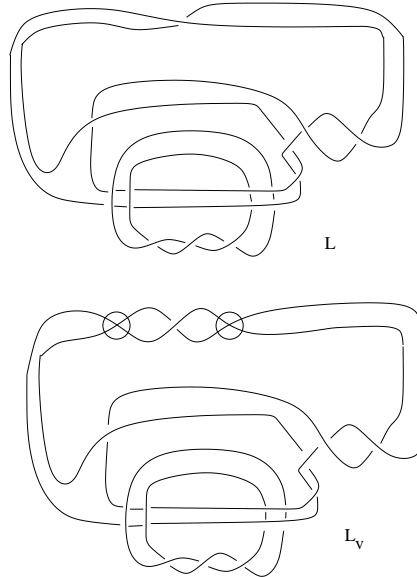
Figure 10: Link Diagrams: L and L_v
