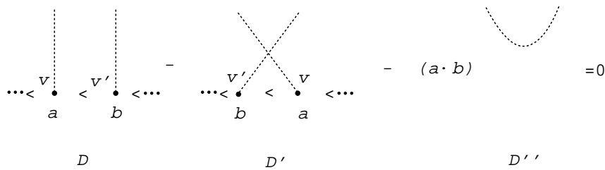
Figure 48: Let D be a uni-trivalent graph and let v < v' be two consecutive univalent vertices in D labeled a, b \in H_1(\Sigma; \mathbf{Z}) . Let D' be the uni-trivalent graph obtained from D by exchanging the order of v and v' . Let D'' denote the uni-trivalent graph obtained from D by connecting two vertices v and v' . Then the ‘‘STU-like relation’’ states that D - D' - (a \cdot b)D'' = 0 , where a \cdot b \in \mathbf{Z} denote the intersection number of a and b . In this figure the univalent vertices are placed according to the total order.
