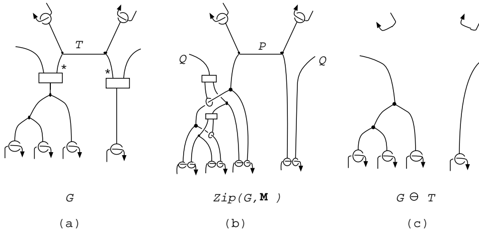
Figure 24: In (a), two asterisks are placed near the two ends of the good input subtree T in G .
