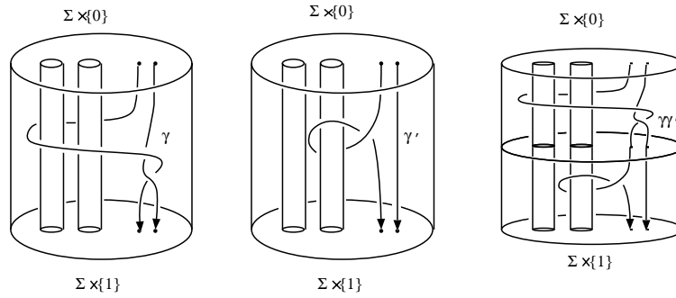
Figure 32: Example of composition of two 2-string links
