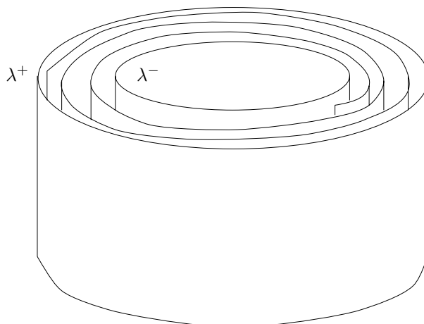
Figure 3: A cylinder is blown up to a foliated cylinder \times I . Then all but the boundary leaves are perturbed to planes. This pocket of leaves lifts to the universal cover to give an annulus of confined directions at infinity without any confined fixed points.
