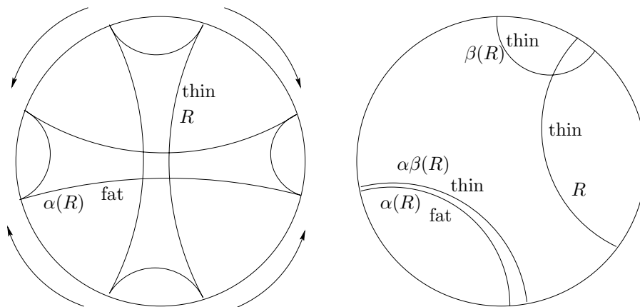
Figure 5: A fat rectangle cannot cross a thin rectangle, or some element would act on S^1 in a weakly pseudo-Anosov manner. Similarly, if a thin rectangle crosses a thin rectangle, a translate of this thin rectangle “protects” fat rectangles from being crossed by fat rectangles.
