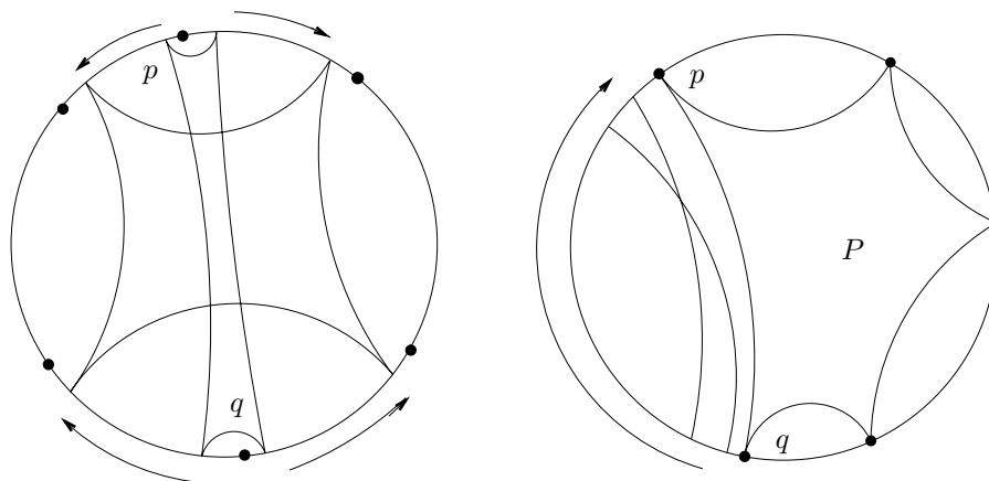
Figure 6: p, q are the vertices of a boundary leaf \gamma of P . If \alpha has at least two fixed points on either side of p, q , the moduli of rectangles nested between these fixed points are bounded above by the action of \pi_1(M) . If \alpha has no fixed points on some side of p, q , the fact that \gamma is not isolated on one side says that some nearby geodesic \gamma_i intersects its translate under \alpha . The solid dots in the figure are fixed points of \alpha . The arrows indicate the dynamics of \alpha .
