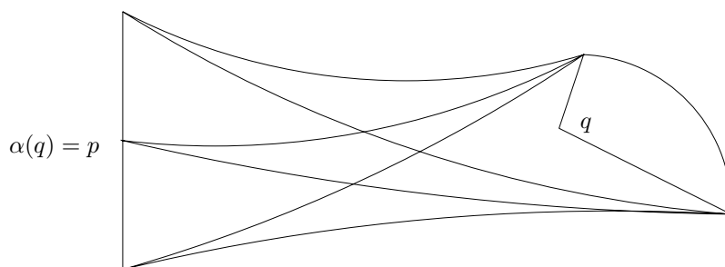
Figure 4: A sufficiently large disk about any point in any leaf is an \epsilon -net for M . By going sufficiently far out towards \mathcal{C} so that the vertical height of H(R) is small, we can find points p, q and \alpha as in the figure.
