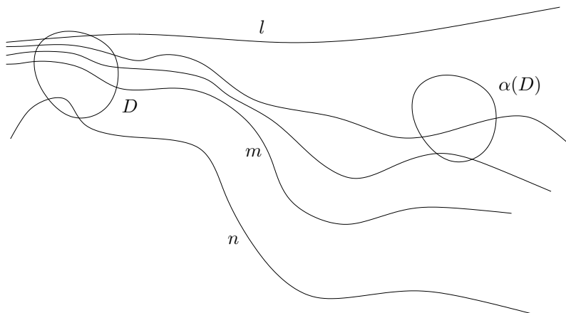
Figure 1: If l is not semi-confined, for any nearby leaf m and any other leaf n , there is an element \alpha \in \pi_1(M) such that \alpha(l) and \alpha(n) are between l and m .
