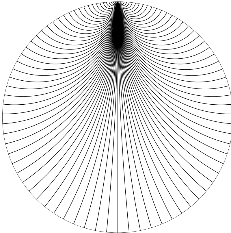
Figure 2: Each \mathbb{H}^2 is foliated by flow lines
