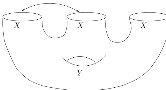
Figure 1: \mathbf{Z}/k -manifold
