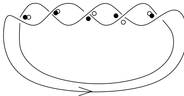
Figure 7: States y and z We have indicated here the two states in absolute degrees 1 and 2. The state z (in dimension two) is indicated by the dark circles, while y is indicated by the hollow ones. It is easy to see that the domain connecting z to y agrees with the domain connecting c to b in the previous picture.
