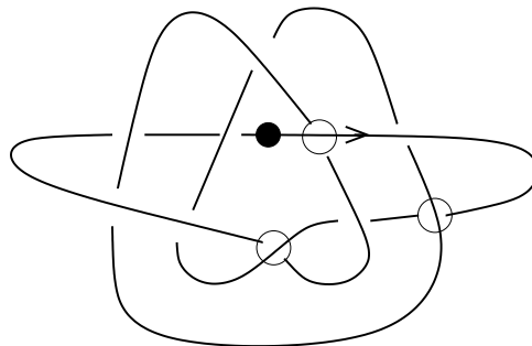
Figure 5: Local Iteration level contributions A decorated knot projection for 10_{161} , showing that it has unknotting number at least 3.
