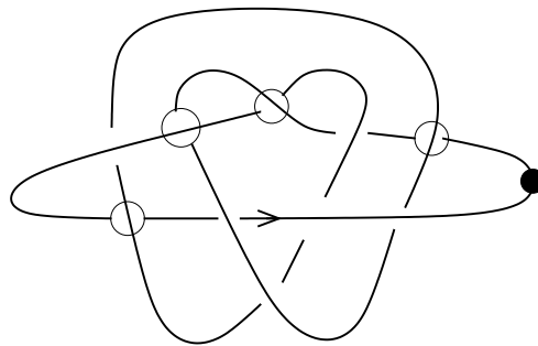
Figure 3: The knot 10_{139} We have circled four crossings: when these are switched, the new knot is the unknot. The black dot indicates the distinguished edge (\circ) used in the decorated knot projection.
