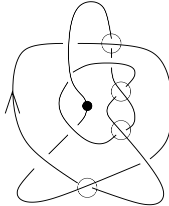
Figure 4: The knot 10_{152} . We have indicated, once again, the crossings needed to unknot 10_{152} , and also the distinguished edge (0, with the dark circle) used in the decorated knot projection for the proof of Proposition 4.3.
