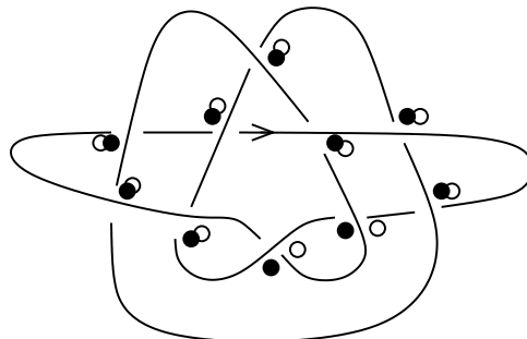
Figure 6: States b and c We have indicated the state c by the dark circles, and b by the hollow ones.
