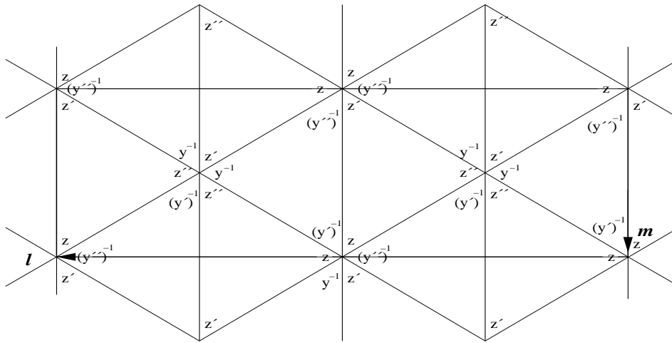
Figure 9: Fundamental domain of the cusp torus, triangulated as the link of the 0–simplex of the ideal triangulation of m004 .
