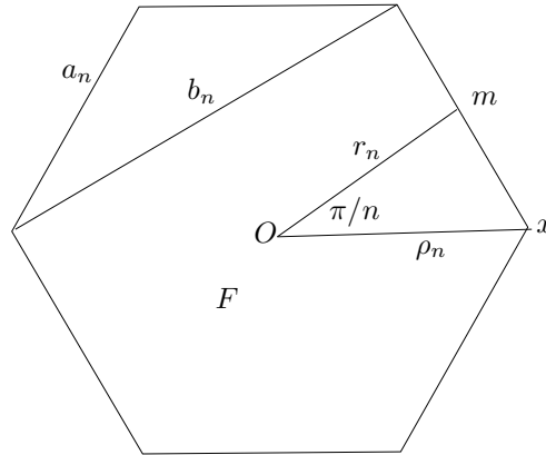
Figure 1: Geometry of a hyperbolic n -gon
