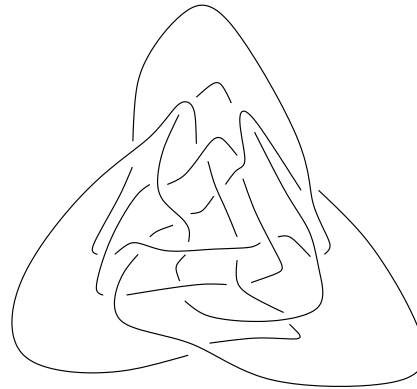
Figure 1.6: L_{2BR} and the Chen's link
