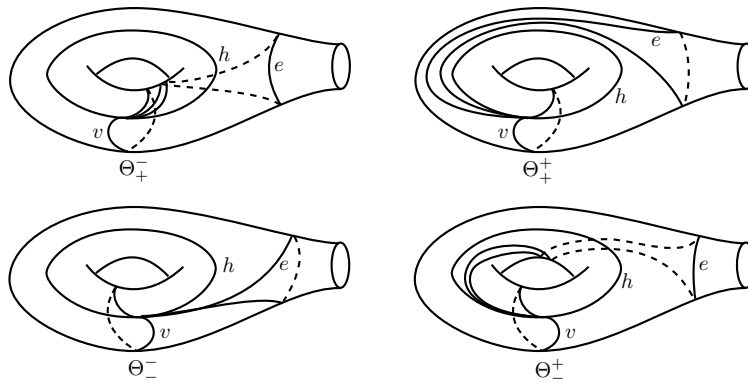
Figure 6: The train tracks \Theta_{\pm}^{\pm}
