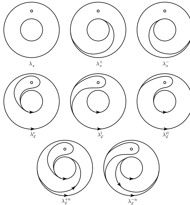
Figure 4: The geodesic laminations containing the simple closed geodesic \lambda_s , as seen in the completion of T - \lambda_s
