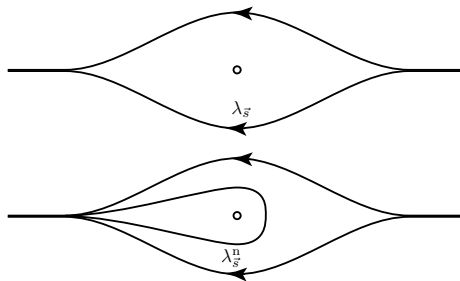
Figure 5: The geodesic laminations \lambda_{\vec{s}} and \lambda_{\vec{s}}^{\text{n}} with \vec{s} irrational, as seen in the completion of T - \lambda_{\vec{s}}
