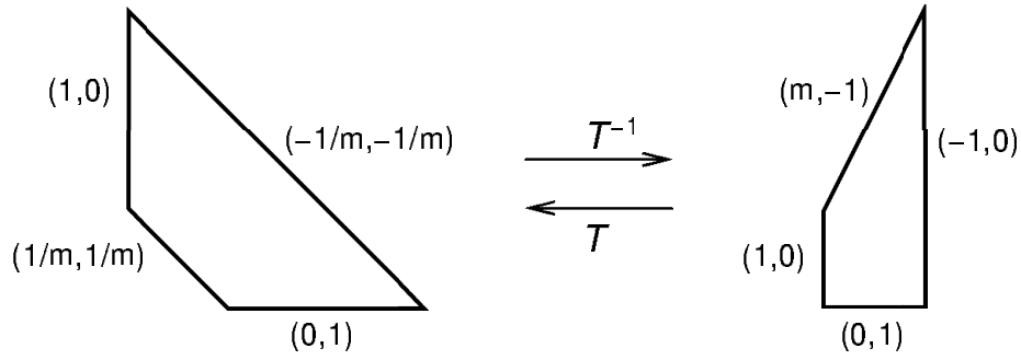
Figure 1. Hirzebruch surfaces.
