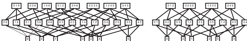
Figure 2: Left: Face poset of \mathcal{F}(\tilde{P}) for the example given in Figure 1, where the solid part is \mathcal{F}(P) . Right: The poset \mathcal{V}(P) . In general, \mathcal{V}(P) is not graded (although it is in this example).
