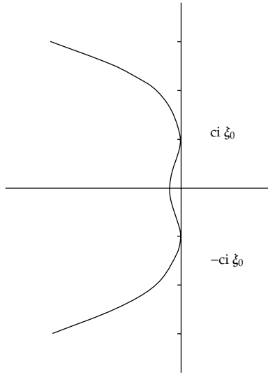
Figure 1: Schematic representation of a possible location of the essential spectrum of the operator L .
