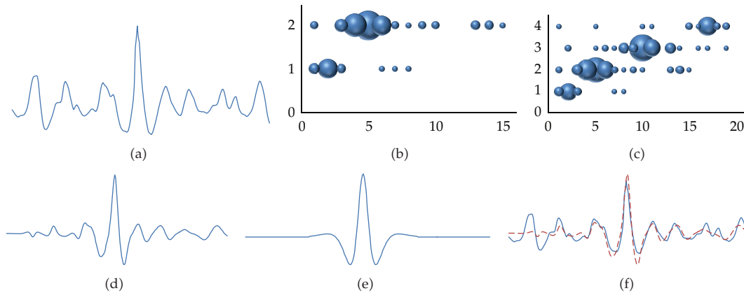
Figure 9: (a) Rogue 1520 from Draupner, January 1995; (b) relative magnitude of coefficients for 3 scales \{1, q, q^2\} for q = 1.5 ; (c) relative magnitude of coefficients for 5 scales \{q^j\}_{j=0}^4 ; (d) {}_q\text{Cos} wavelet approximation using largest 30 coefficients; (e) largest magnitude of {}_q\text{Cos} ( q = 1.5 , scale = q^2 , shift = 5 \cdot b = 12.2 ); (f) comparison between Draupner data and {}_q\text{Cos} wavelet reconstruction.
