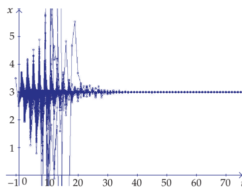
Figure 11: Stable equilibrium point \hat{x} = 3 for p = 4 , q = -1 , \sigma = 0.5 .
