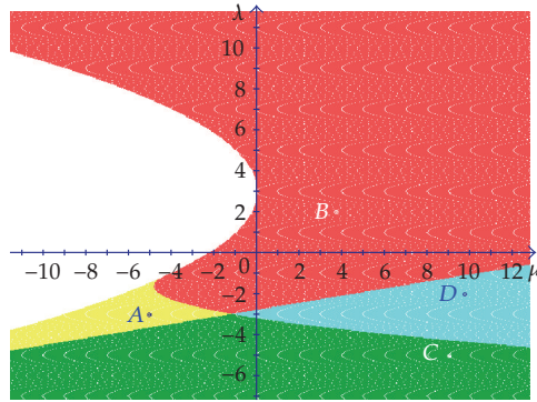
Figure 1: Stability regions, \sigma^2 = 0 .
