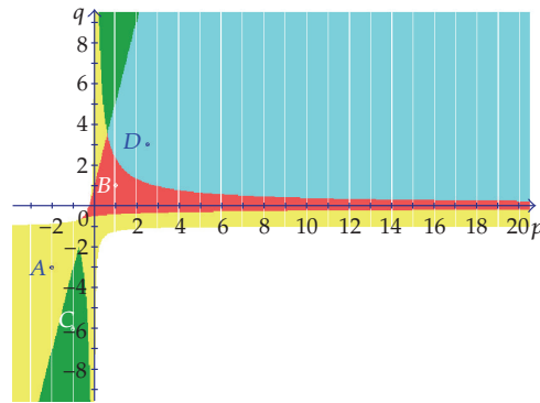
Figure 15: Stability regions, \sigma = 0 .
