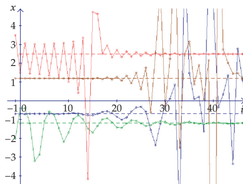
Figure 10: Stable equilibrium points \hat{x} = 2.5 and \hat{x} = -1.2 , unstable \hat{x} = 1.2 and \hat{x} = -0.7 .
