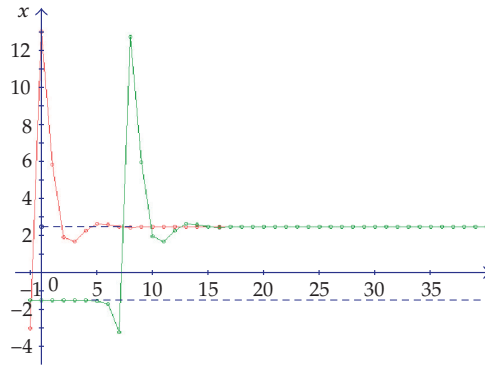
Figure 6: Stable equilibrium point \hat{x}_1 = 2.5 and unstable \hat{x}_2 = -1.5 for \mu = 3.75, \lambda = 2 .
