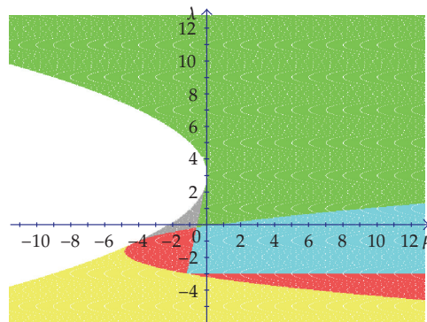
Figure 4: Stability regions, \sigma^2 = 0 .
