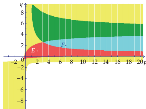
Figure 16: Stability regions, \sigma = 0.7 .
