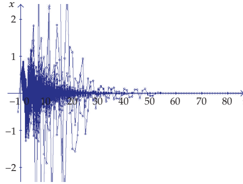
Figure 13: Stable equilibrium point \hat{x}_2 = 0 for \mu = 0, \lambda = -2, a = 1, \sigma = 0.6 .
