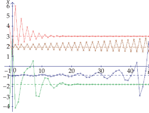
Figure 9: Stable equilibrium points \hat{x} = 3 and \hat{x} = -1.8 , unstable \hat{x} = 1.93 and \hat{x} = -0.9 .
