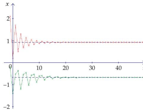
Figure 20: Stable equilibrium points \hat{x}_1 = 0.925 and \hat{x}_2 = -0.675 for p = 2.5, q = 3 .
