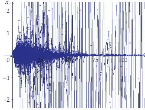
Figure 14: Unstable equilibrium point \hat{x}_2 = 0 for \mu = 0 , \lambda = -2 , a = 1 , \sigma = 0.9 .
