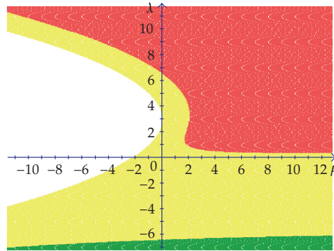
Figure 3: Stability regions, \sigma^2 = 0.8 .
