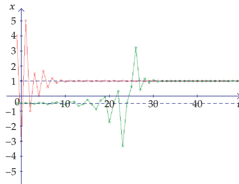
Figure 18: Stable equilibrium point \hat{x}_1 = 1 and unstable \hat{x}_2 = -0.5 for p = 1, q = 1 .
