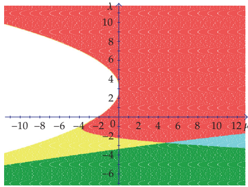
Figure 2: Stability regions, \sigma^2 = 0.3 .
