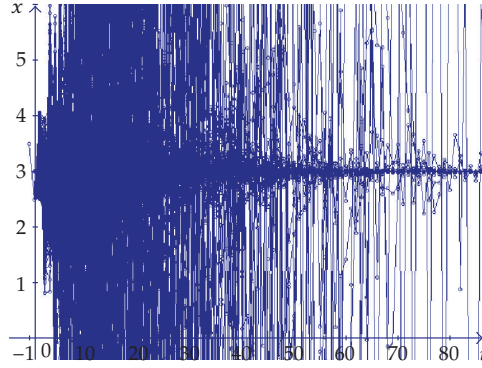
Figure 12: Unstable equilibrium point \hat{x} = 3 for p = 4, q = -1, \sigma = 0.9 .
