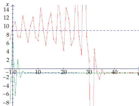
Figure 7: Unstable equilibrium point \hat{x}_1 = 9 and stable \hat{x}_2 = -1 for \mu = 9 , \lambda = -5 .
