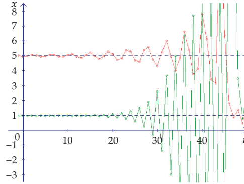
Figure 5: Unstable equilibrium points \hat{x}_1 = 5 and \hat{x}_2 = 1 for \mu = -5, \lambda = -3 .
