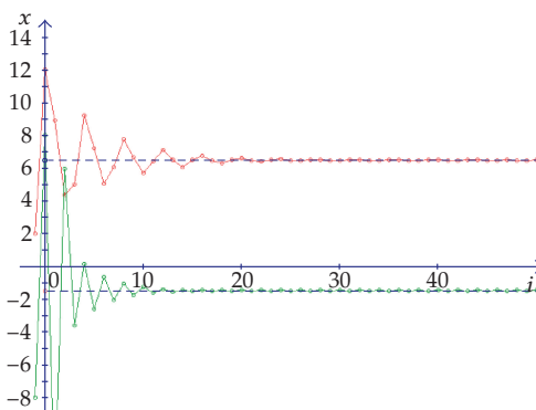
Figure 8: Stable equilibrium points \hat{x}_1 = 6.5 and \hat{x}_2 = -1.5 for \mu = 9.75 , \lambda = -2 .
