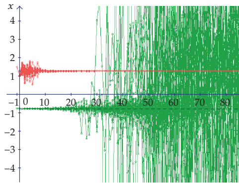
Figure 21: Stable equilibrium points \hat{x}_1 = 1.281 and \hat{x}_2 = -0.781 for p = 2, q = 1, \sigma = 0.7 .
