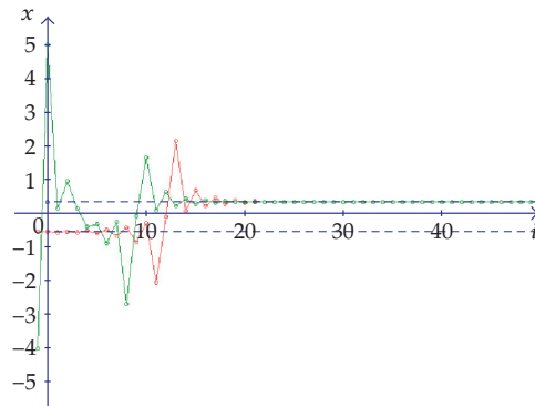
Figure 19: Unstable equilibrium point \hat{x}_1 = -0.558 and stable \hat{x}_2 = 0.358 for p = -1, q = -6 .
