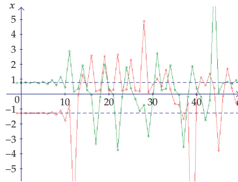
Figure 17: Unstable equilibrium points \hat{x}_1 = -1.281 and \hat{x}_2 = 0.781 for p = -2, q = -3 .
