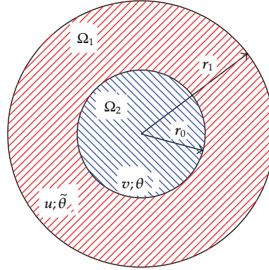
Figure 1: Domains \Omega_1 and \Omega_2 and boundaries of the transmission problem.
