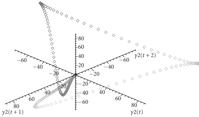
Figure 5.10. The time series for \varepsilon(\tau) on a three-dimensional space corresponding to shift by 40 time steps.
