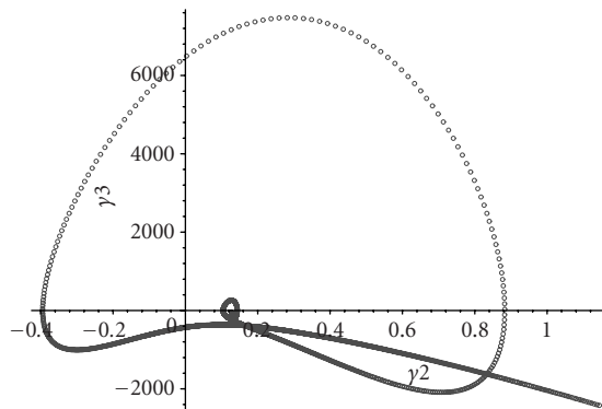
Figure 5.4. This curve is a magnification of the motion in the neighborhood of the endpoint of Figure 5.3 , starting below the axis and moving to the left. It makes another loop and ends in a smaller pattern.
