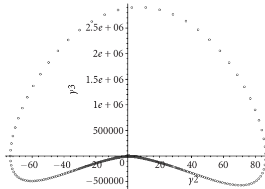
Figure 5.3. This curve continues the evolution within the attractor, starting in the neighborhood of the origin, winding up and around to the right, and terminating almost at the same point (a little above), coming in from the right.
