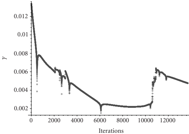
Figure 5.8. The largest averaged Lyapunov exponent (the values must be divided by the size of the interval 10^{-7} ) as a function of the accumulated \tau . We have used interval 0.4 \times 10^{-6} . Note the sharp jump at approximately 10,400 steps, indicating the development of a very large instability in this neighborhood (the additional terms here are divided by 10^4 , the number of time steps).
