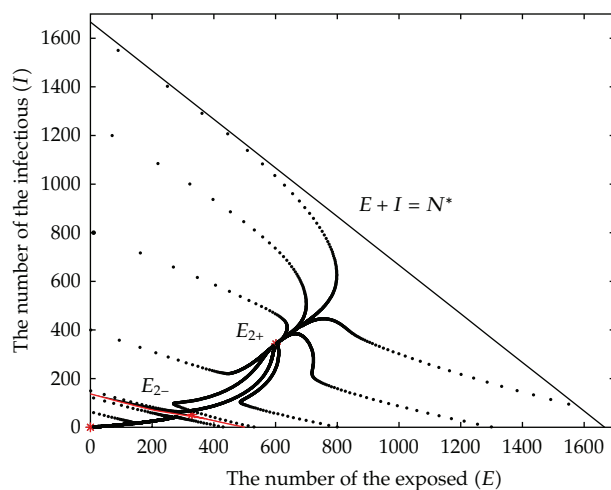
Figure 3: The attraction separatrix for those two equilibria of model (3.1).
