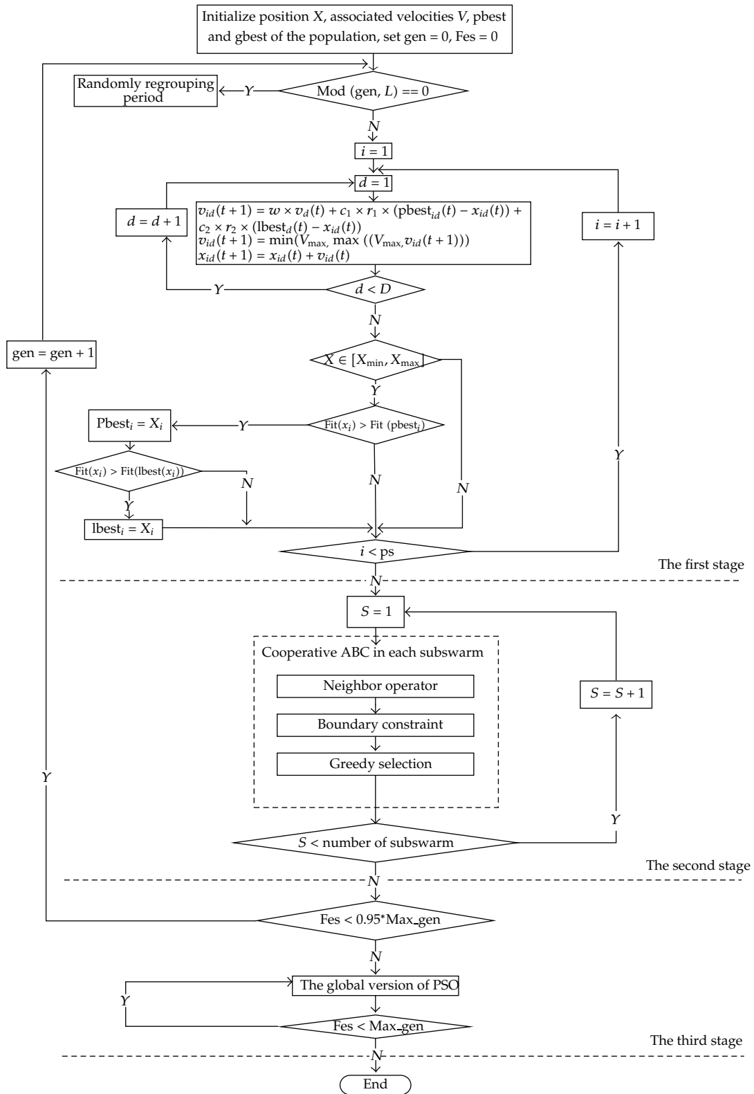
Figure 3: The flowchart of the DM-PSO-ABC.
