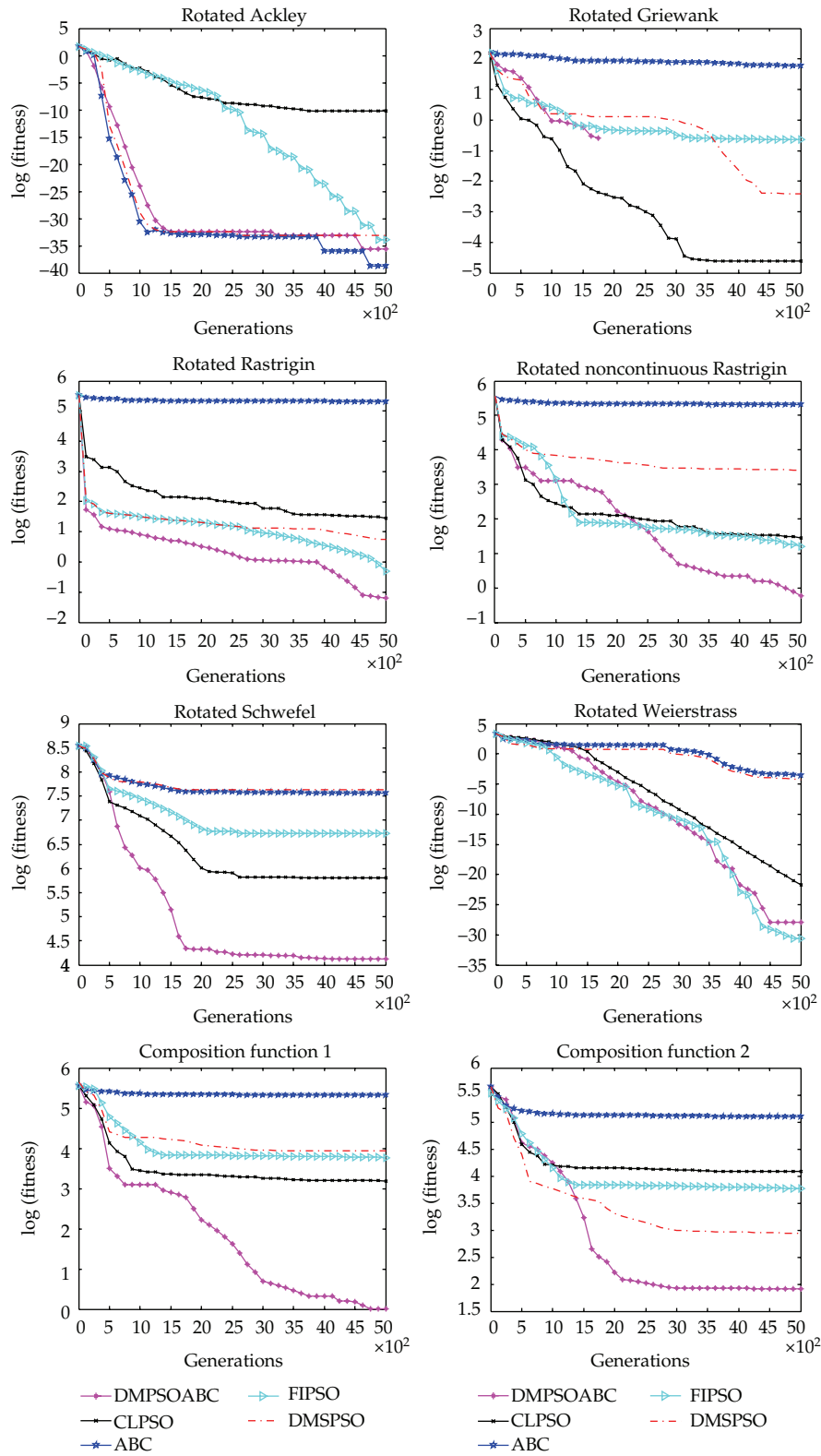
Figure 4: The median convergence characteristics of 30-D test functions.
