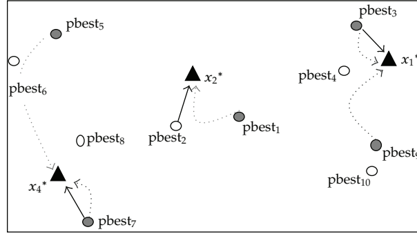
Figure 2: Illustration of local search phase for a population with 10 particles.
