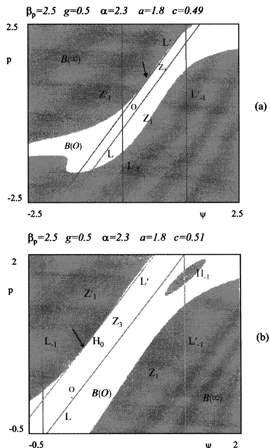
FIGURE 2 Basin bifurcations of the stable fixed point O=(0,0) , observed in the regime of noninvertibility of the map T , for \beta_p=2.5, g=0.5, \alpha=2.3, a=1.8 and by increasing c from the value 0.49. As explained in the text, the critical curves of the map allow one to explain the qualitative changes in the basin structure. At c=0.49 in (a), where the basin of the origin, the white region \mathcal{B}(O) , is a simply connected area. At c=0.51 in (b) and (c), where the grey region \mathcal{B}(\infty) crosses the critical curve L' , entering the region Z_3 and \mathcal{B}(O) is a multiply connected area. At c=0.533 in (d), where a new crossing of the boundary L causes the appearance of new holes. A different dynamic effect is associated with a similar crossing by the hole S_{-1} : in (e), where c=0.534 , it is shown that differently from the previous cases the hole Q_{-1} generated by the new crossing is now in the region Z_3 , and thus it has three distinct rank-1 preimages, each of which has one or three preimages, so that a drastic increase in the numbers of the holes is observed, leading to an increasing complexity in the structure of the basin \mathcal{B}(O) . This kind of bifurcation also occurs in a “backward” way, with the effect of decreasing the number of holes, as shown in (f), obtained for c=0.55 .
