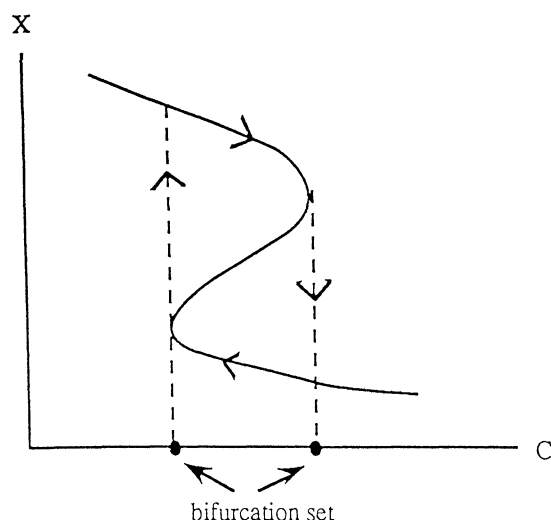
FIGURE 1 Fold catastrophe.
