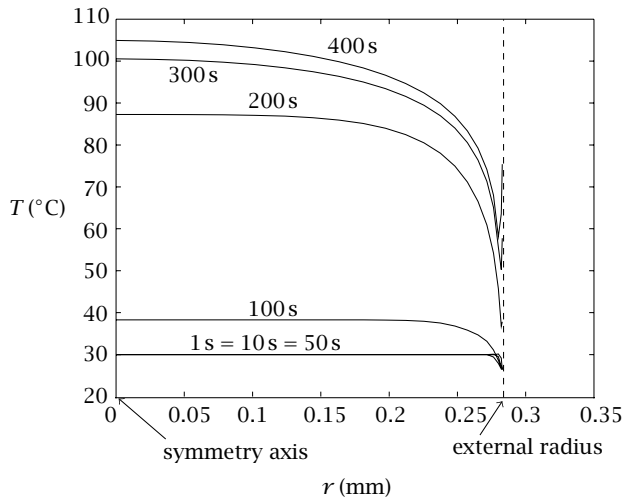
FIGURE 5.6. Radial temperature profile at z = 0 .
