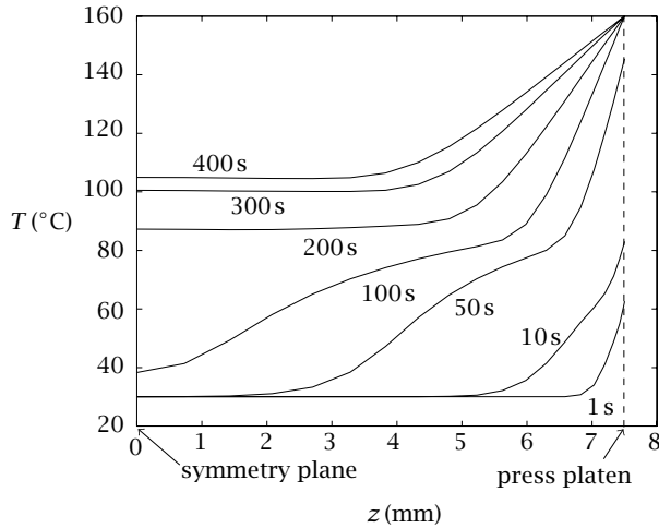
FIGURE 5.2. Axial temperature profile at r = 0 .
